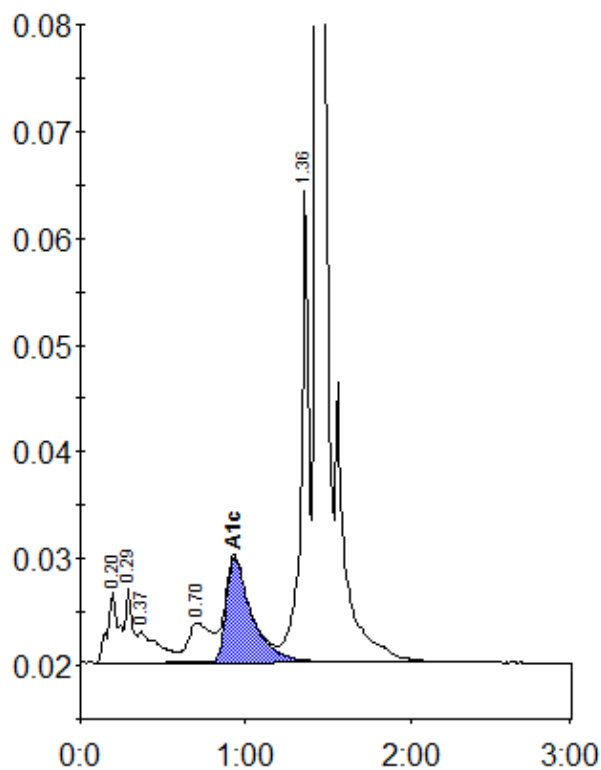
Peak table - ID: 10528460
